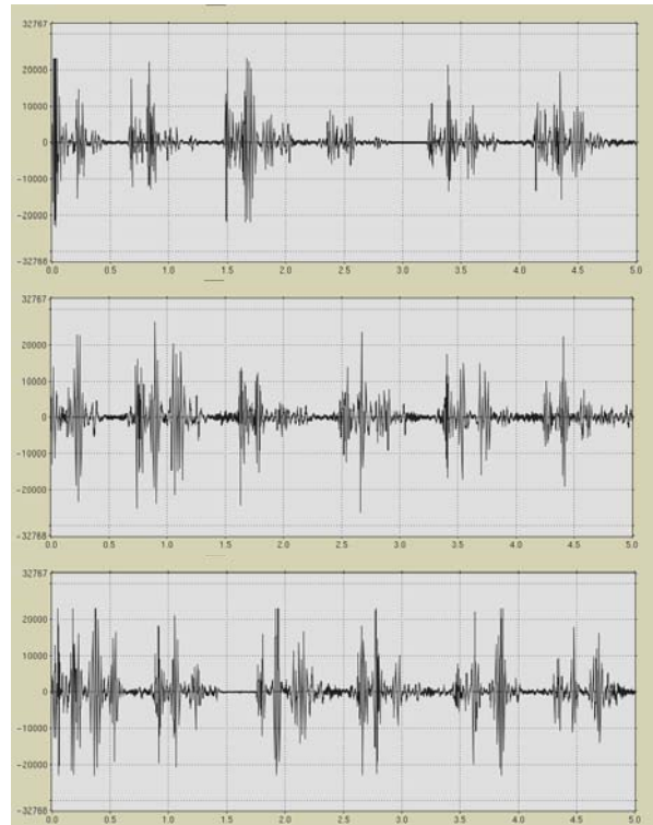
Figure 6. Same as Fig. 4, measured with the dual-mode stethoscope in the active ultrasound-Doppler mode.
